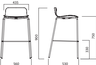
SG280L STOOL
