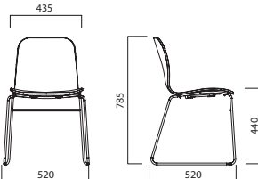
S280L SLED
