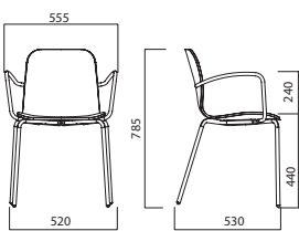
S280L 4 LEGS WITH ARMS
