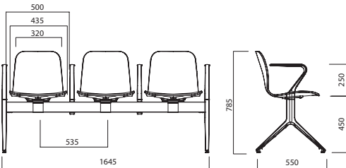
TR280L ON CORE BENCH
