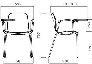
S280L 4 LEGS WITH TABLET
