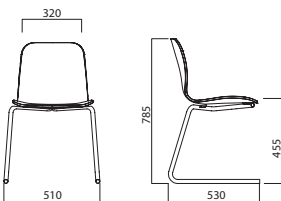
S280L REVERSE CANTILEVER
