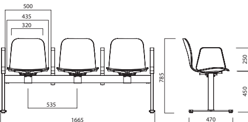
TR280L ON LINEAR BENCH
