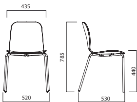
S280L 4 LEGS
