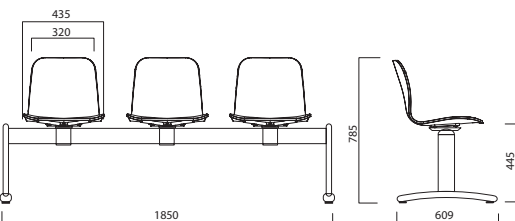
TR280L ON 500 BENCH
