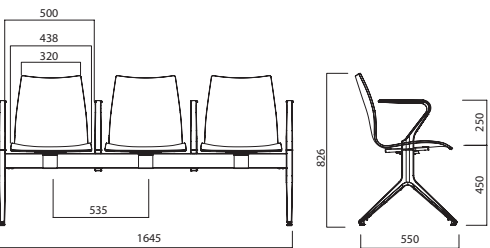
TR290L ON CORE BENCH
