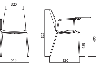
S290L 1BTS 4 LEGS WITH TABLET
