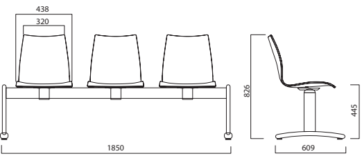
TR290L ON 500 BENCH
