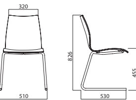
S290L SLRC REVERSE CANTILEVER
