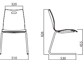
S290L SLRC REVERSE CANTILEVER ALU
