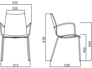
P290L 4 LEGS WITH ARMS
