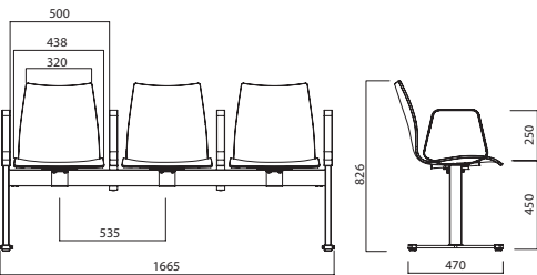
TR290L ON LINEAR BENCH
