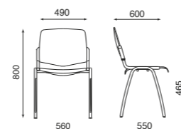
S1900F e S1900T 4 LEGS
