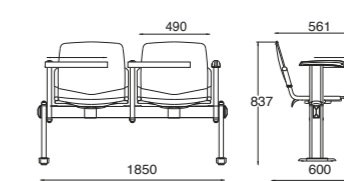
TR1900 BENCH FOR UPHOLSTERY - OVERTURNABLE SEAT
