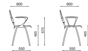
S1900 4 LEGS WITH ARMS
