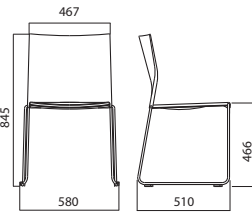
S220L SLED WOOD
