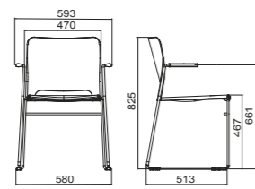
P221 WITH ARMS
