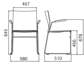
P220 WITH ARMS
